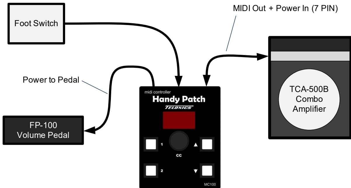
Fig 2 - Handy Patch used with the TCA-500B Combo and FP-100 Volume Pedal
